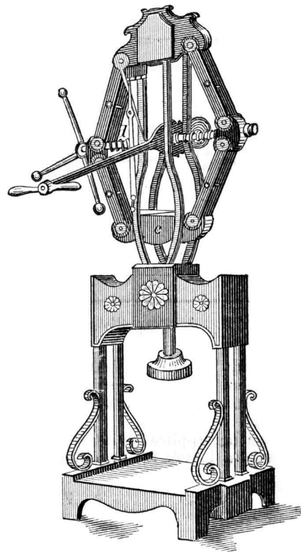
Toggle-Press.
