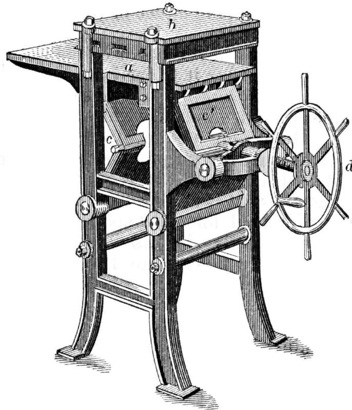
Toggle-Press.
